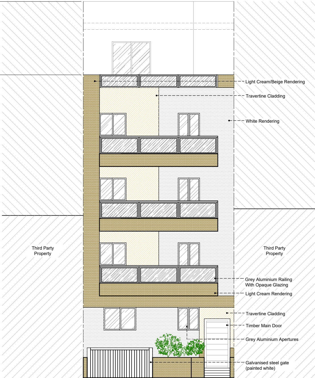
PROPOSED ELEVATION
